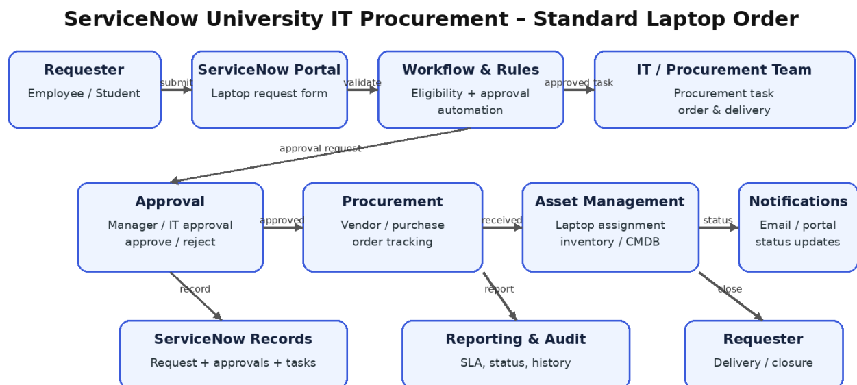
Figure 1: Solution architecture and data flow for the ServiceNow university IT procurement automation
